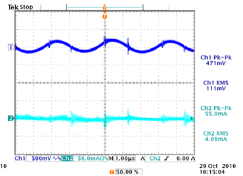
Input/Output ripples of UH2H280abcd-S18XXX ( V_{IN} : 270V, Load: 18A, L_{IN} =20uH, C_{IN} =270uF) (External CAP100uF/100V)
