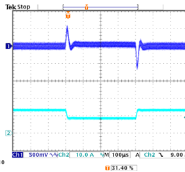
Transient response of UH2H280abcd-S18XXX ( V_{IN} : 270V, Load: 14.5A/7.5A@2.5A/μS) (External CAP100uF/100V)
