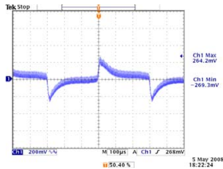
Transient response of UH48050abcd-NA0xxx ( V_{IN} : 50V, Load: 70.0A/50.0A@2.5A/ \mu S)
