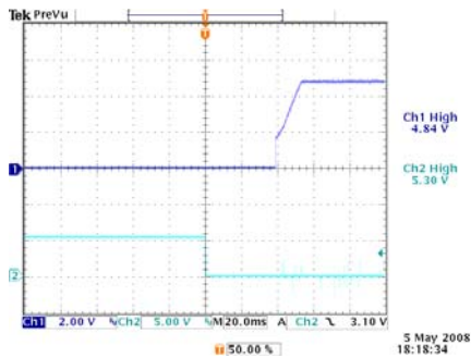
Start-up waveform of UH48050abcd-NA0xxx ( V_{IN} : 50V, Load: 100A)
